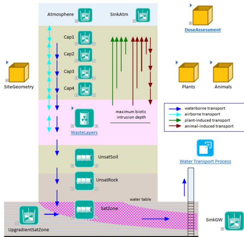
Figure 5: Near surface radioactive waste disposal system.
