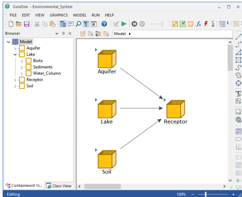
Figure 3: Total-system model including submodels for the aquifer, lake, soil, and receptor systems.
